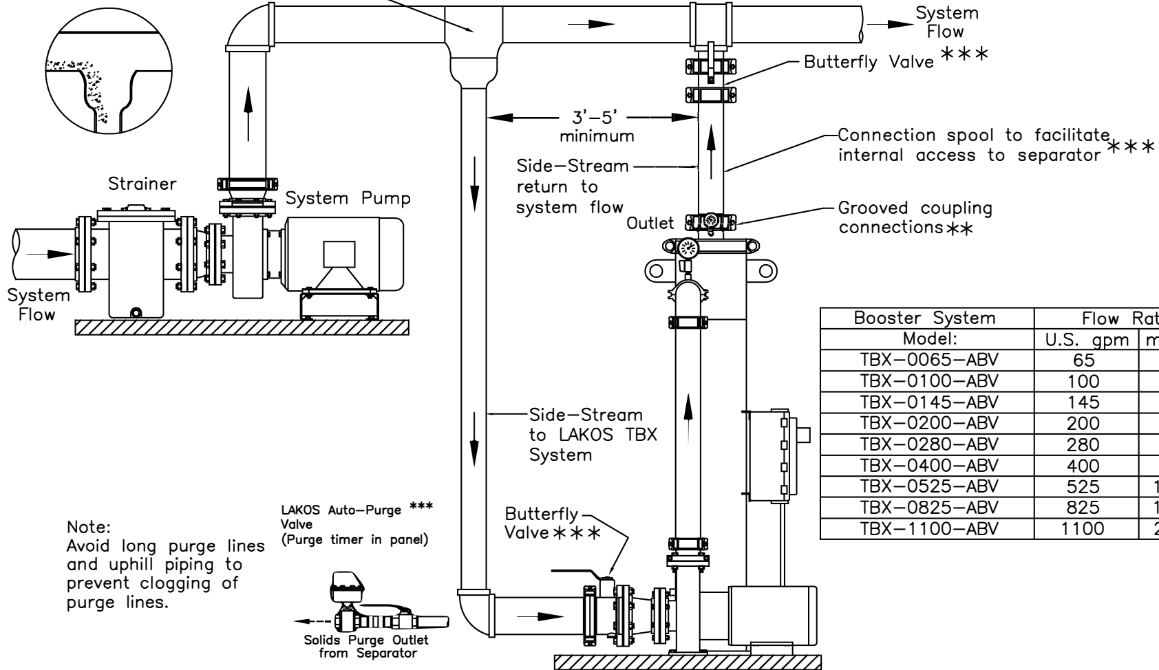
LAKOS TBX Booster System with Auto-Purge
